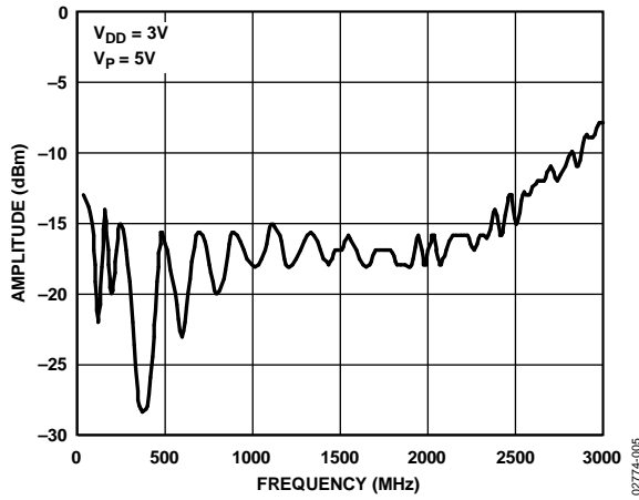
Figure 5. Input Sensitivity (RF Input)
