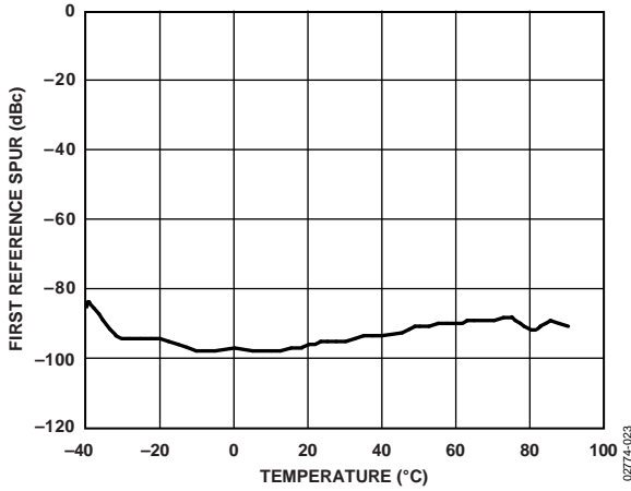
Figure 23. RF Spurs vs. Temperature
